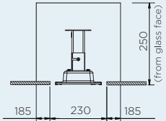
OPTION 2 - NARROW CAVITY SPACE
