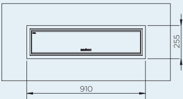
MINIMUM CAVITY SIZE FOR BOTH 2300W & 3400W MODELS
